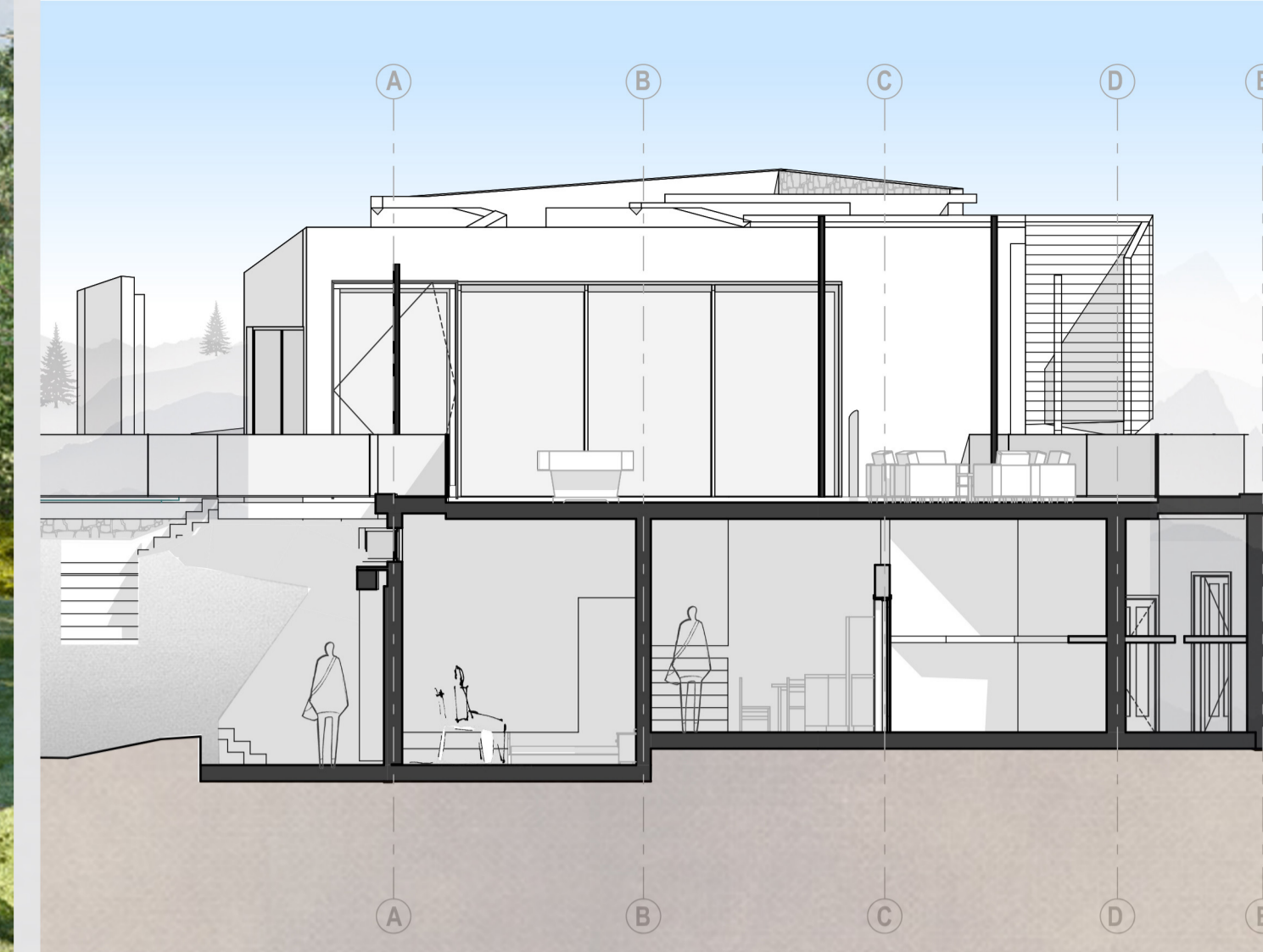
Section through the main entrance lobby looking towards the entertainment area
